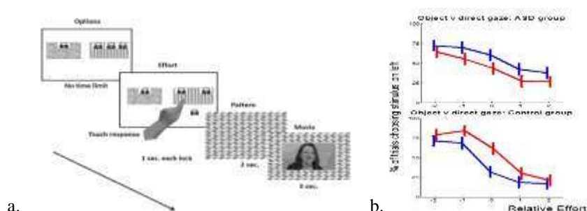
Figure 2: a) Trial structure of the Choose A Movie (CAM) task. b) Results comparing adults with and without autism on the CAM task (figures adapted from [7,8]). The results show logistic regression analysis with relative cost (as addition key presses) on the x axis and percentage of preference for stimuli on left on Y axis. The red line show social stimuli and blue line shows the object stimuli.
